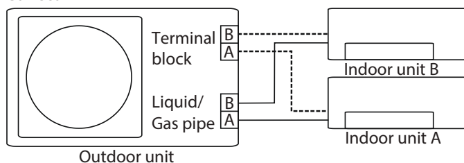
Incorrect wiring
